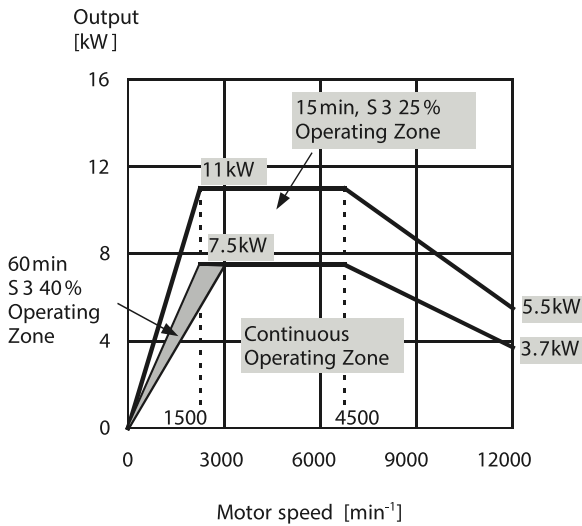
MA-645/745/850 Fanuc-Driver
