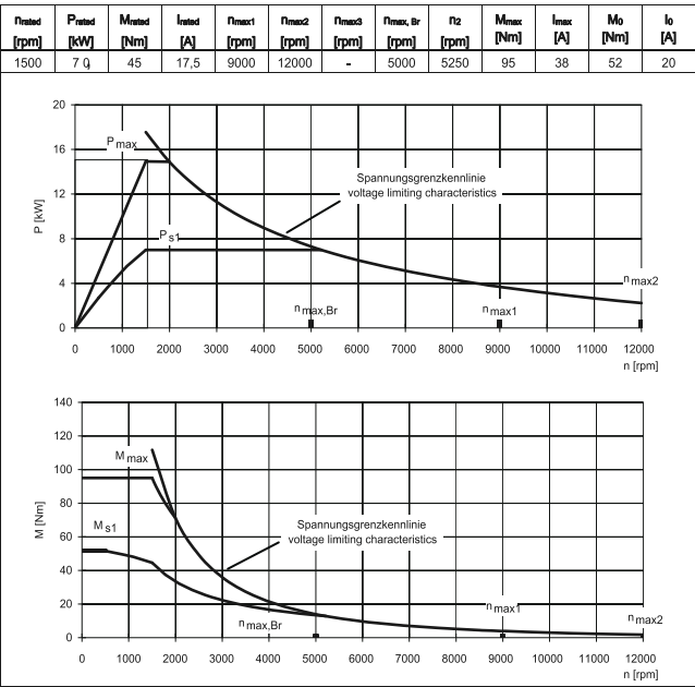
MA-645/745/850 Siemens-Driver
